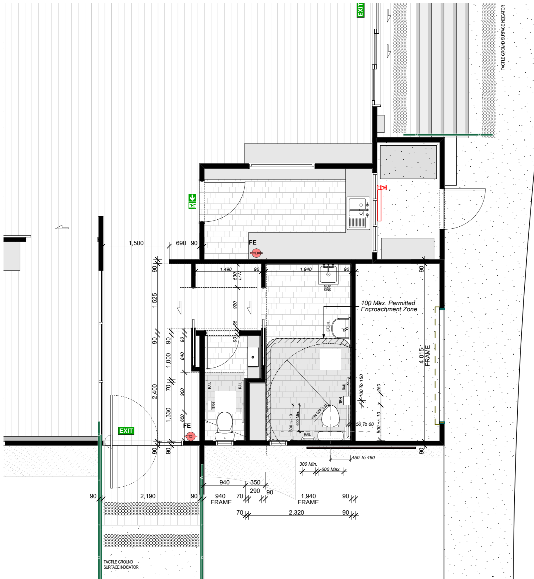
ACCESSIBILITY PLAN 1:50
