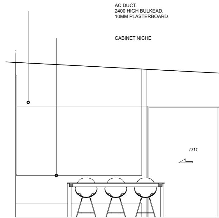
BOARD ROOM 1 1:50
