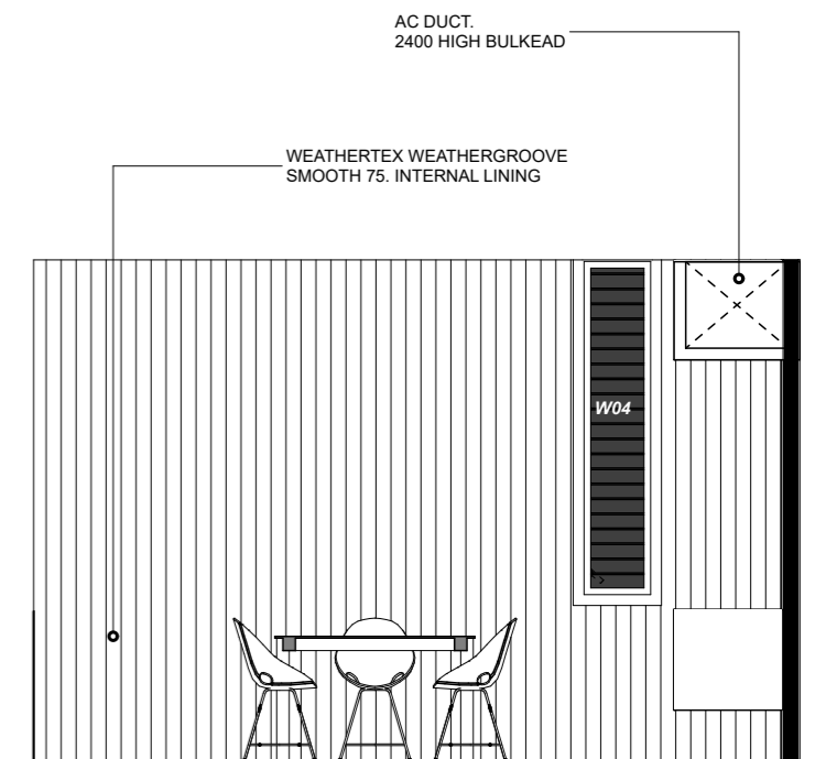
BOARD ROOM 4 1:50
