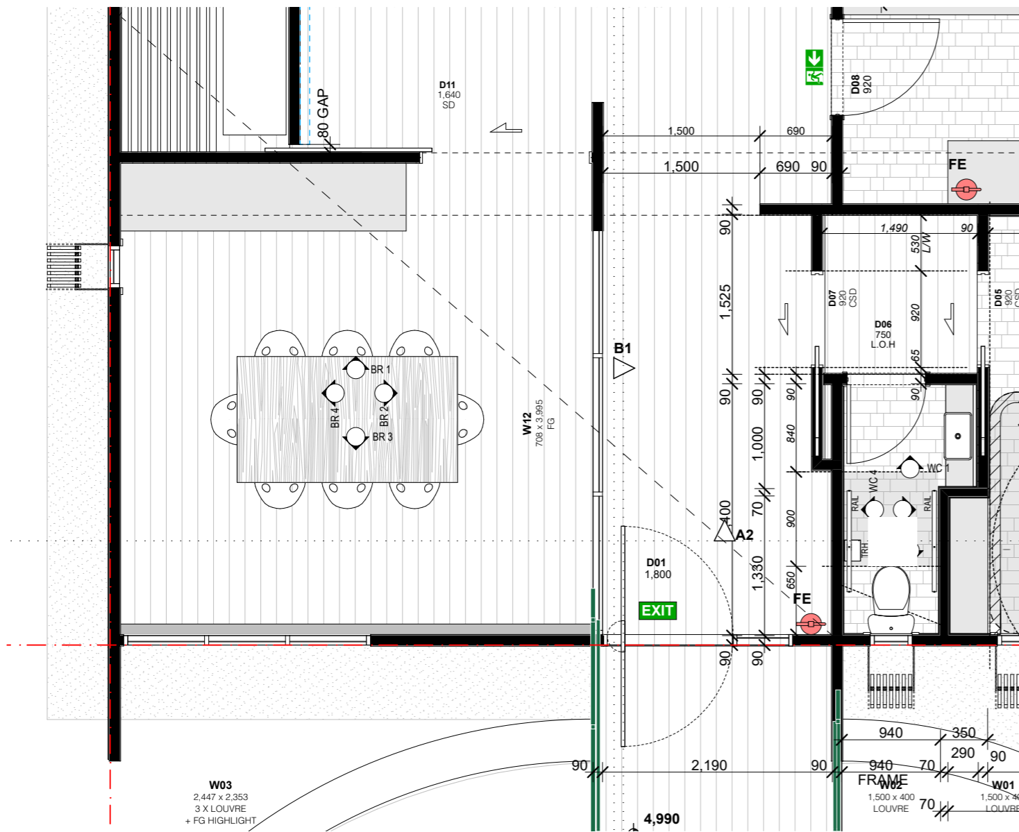
BOARD ROOM FLOOR PLAN 1:50
