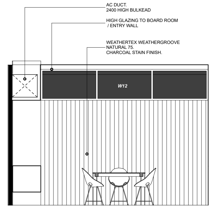
BOARD ROOM 2 1:50
